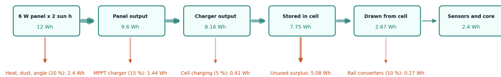
Figure 4. Daily energy flow in the worst month at the 100 mW design allowance (FND-CAL-001).
