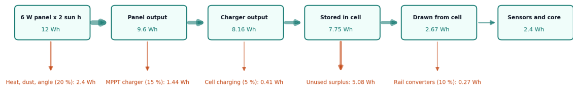
Figure 4. Daily energy flow in the worst month at the 100 mW design allowance (FND-CAL-001).
