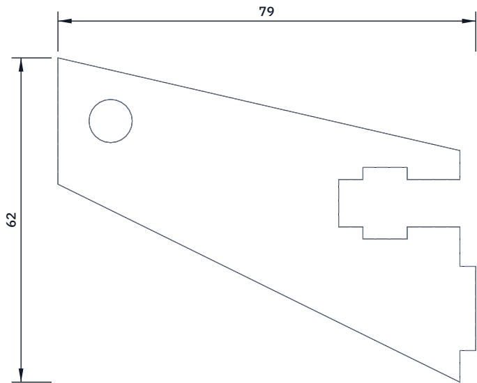
TOP VIEW Scale 1:1; looking down (along -Z)
