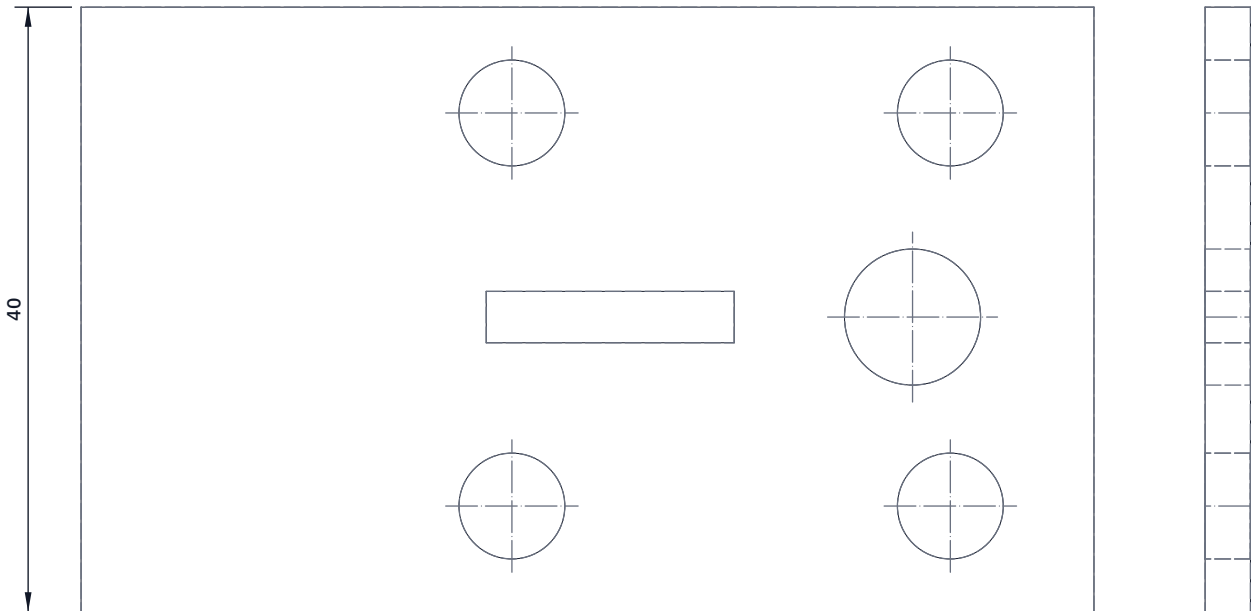
FRONT VIEW Scale 2:1; looking at the front (along +Y)
