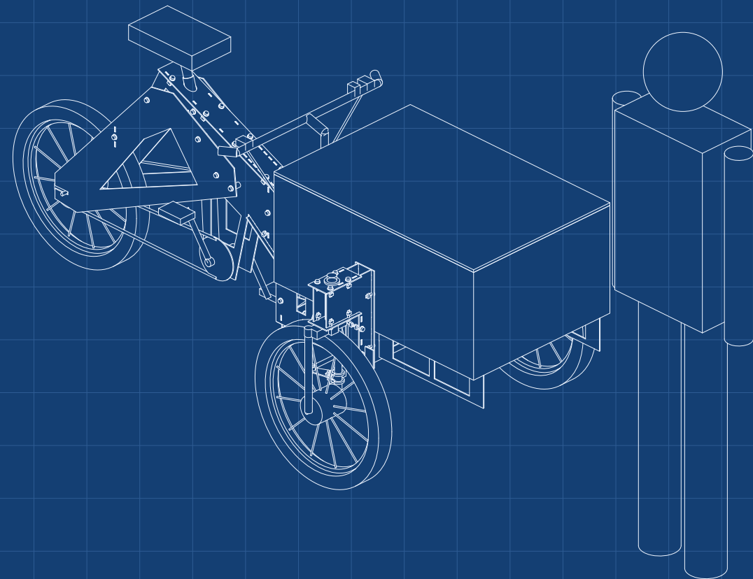
ISOMETRIC VIEW
