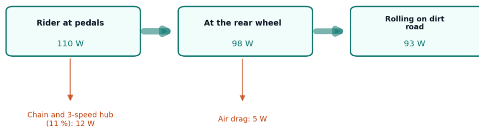
Figure 2. Where 110 W of rider power goes at 301.2 kg gross on a flat dirt road (FTK-CAL-001 section 4). All values are estimates.
