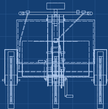
RIGHT VIEW Scale 1:20
