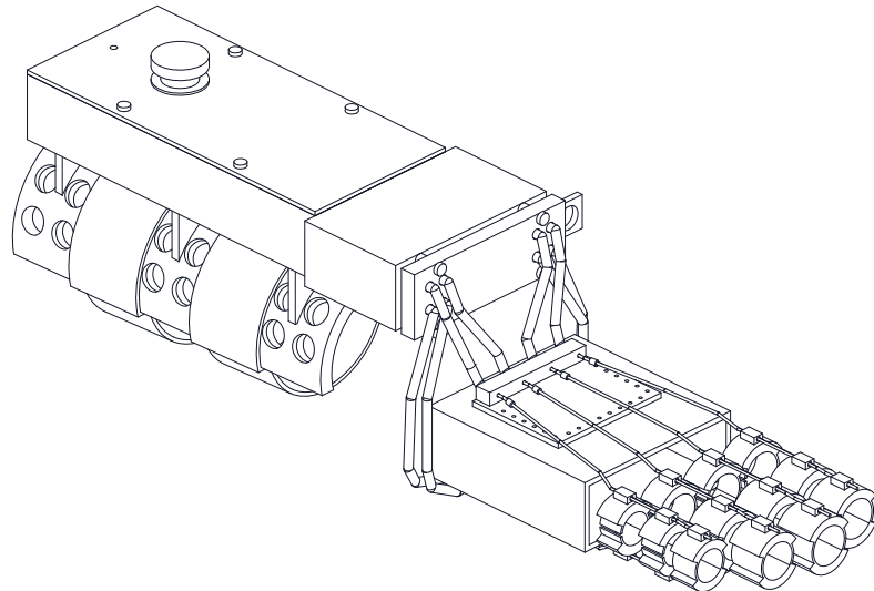
ISOMETRIC VIEW, WHOLE DEVICE
