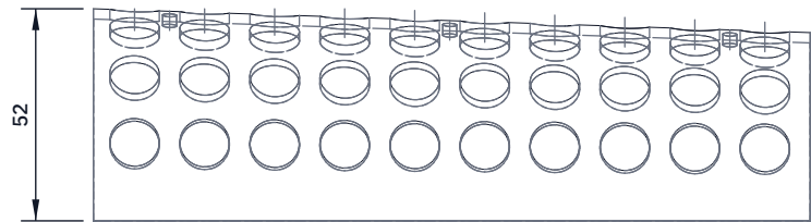
FRONT VIEW Scale 1:2; looking at the front (along +Y)
