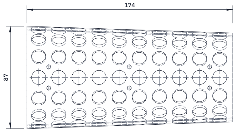
TOP VIEW Scale 1:2; looking down (along -Z)
