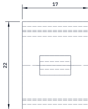
TOP VIEW Scale 2:1; looking down (along -Z)
