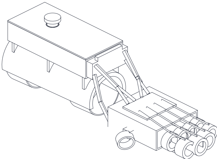
ISOMETRIC VIEW, WHOLE DEVICE Left hand shown (mirror of the modeled right hand); not to scale
