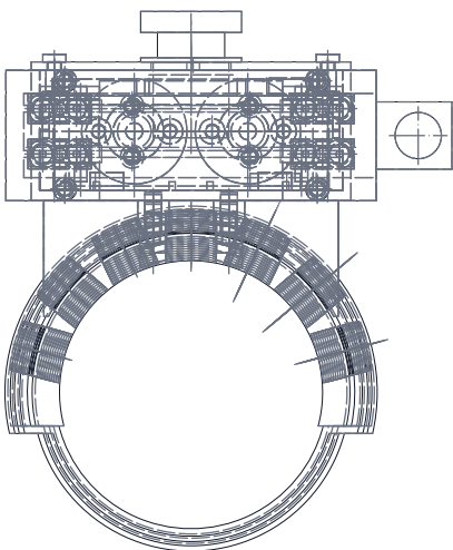
RIGHT VIEW
