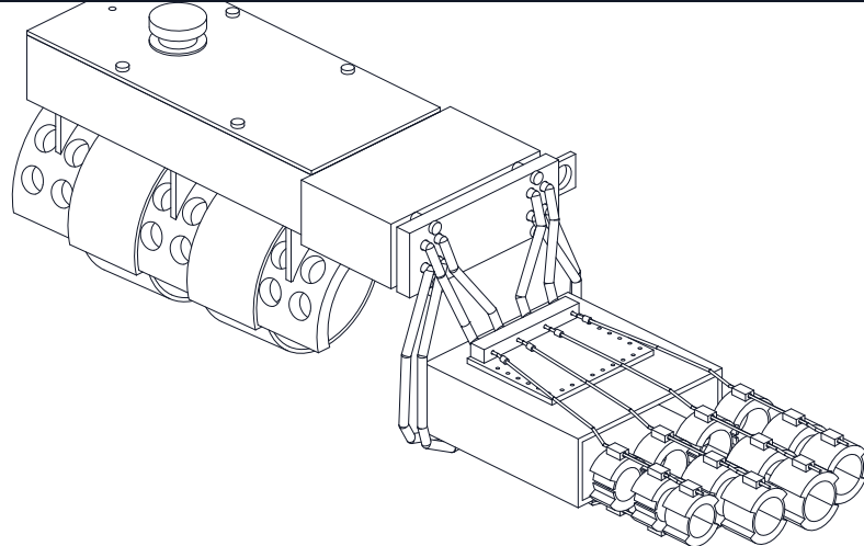
ISOMETRIC VIEW, WHOLE DEVICE
