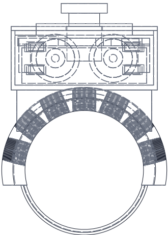
RIGHT VIEW Scale 1:2
