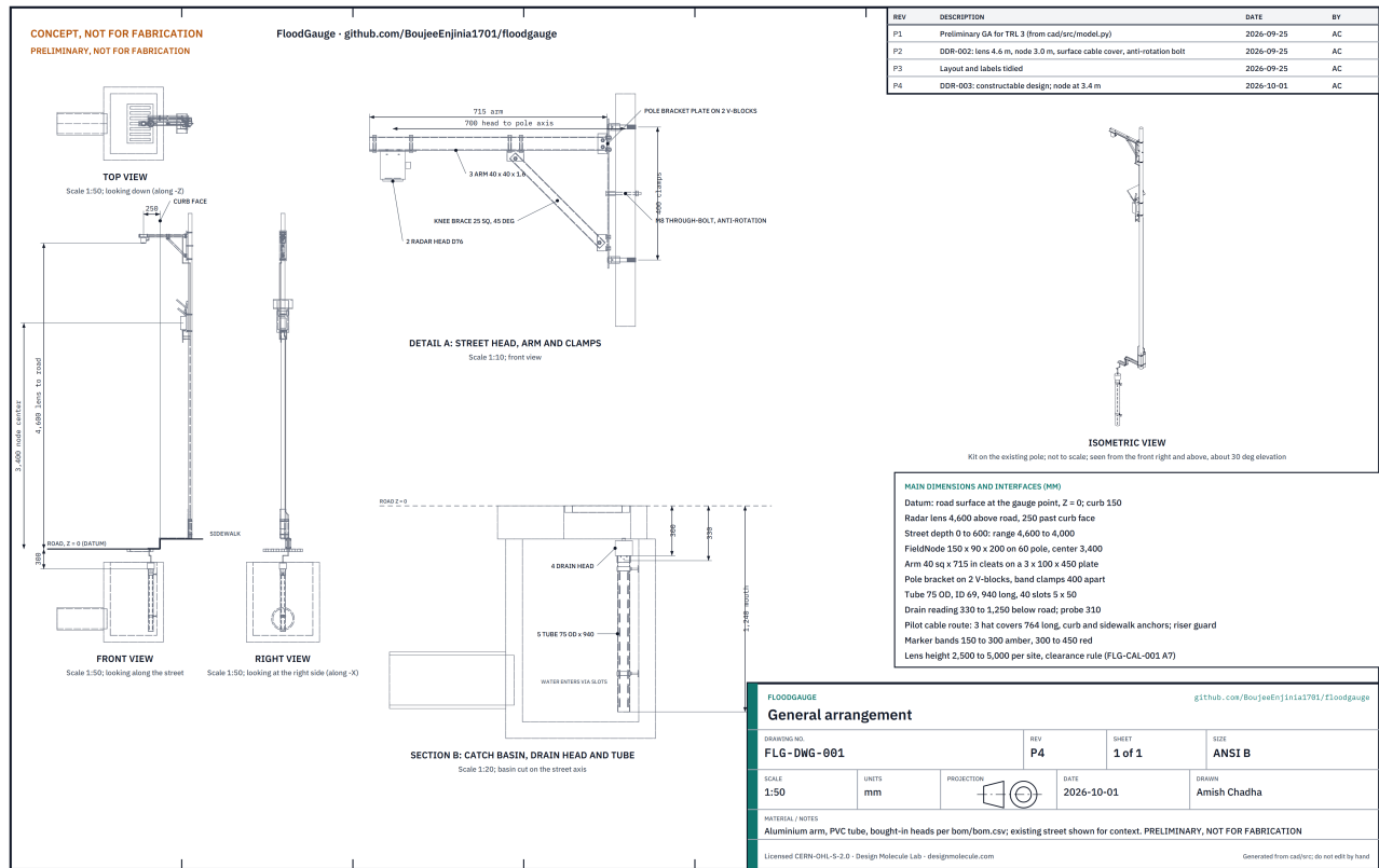
Figure 5. General arrangement FLG-DWG-001, Rev P4, from cad/src/model.py . PRELIMINARY, NOT FOR FABRICATION.
