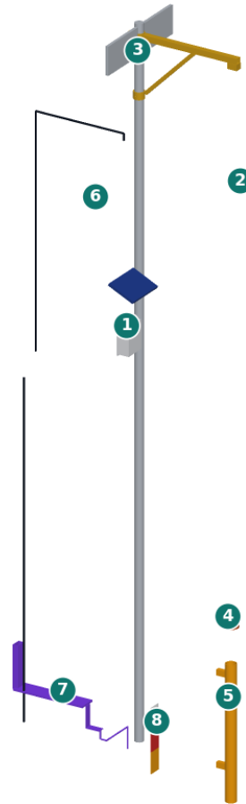
Figure 4. Exploded view with BOM numbers. The existing street and basin are not shown.
