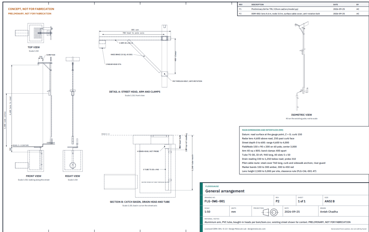
Figure 5. General arrangement FLG-DWG-001, Rev P2, from cad/src/model.py . PRELIMINARY, NOT FOR FABRICATION.
