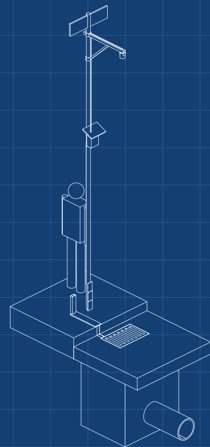
ISOMETRIC VIEW Not to scale; grey is for scale; seen from the front right and above, about 30 deg elevation
