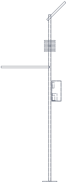
DETAIL B: MAST AND CONTROLLER Scale 1:25, radial view
