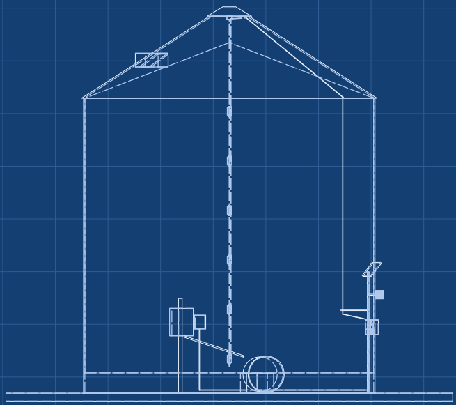
FRONT VIEW Scale 1:100
