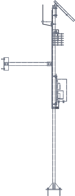
DETAIL B: MAST AND CONTROLLER
