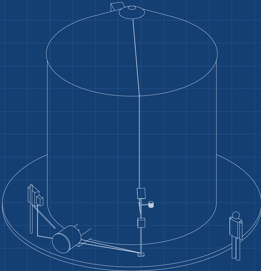
ISOMETRIC VIEW
