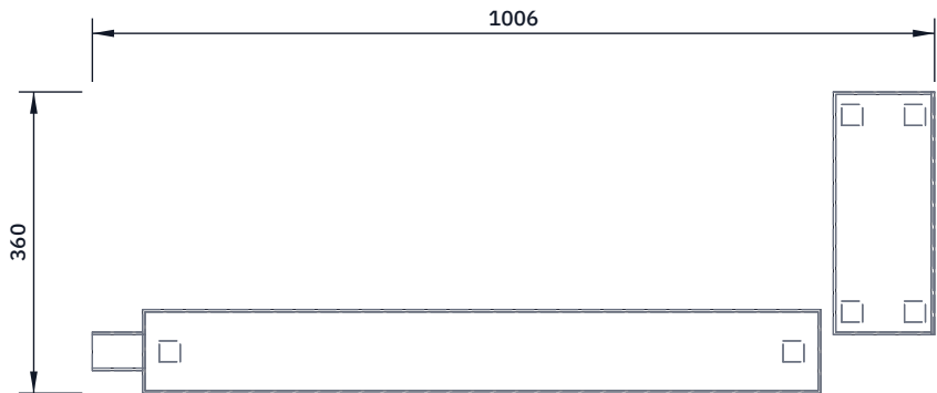
TOP VIEW Scale 1:10; looking down (along -Z)
