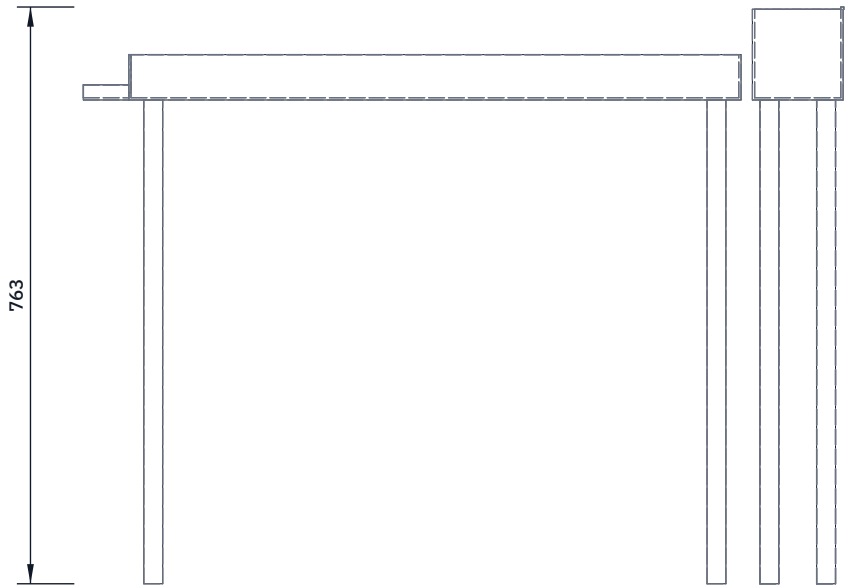
FRONT VIEW Scale 1:10; looking at the front (along +Y)
