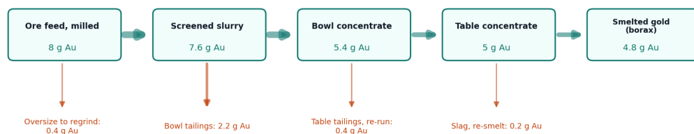
Figure 2. Gold balance for one 8 h shift at 200 kg/h on a reference ore of 5 g/t (GVS-CAL-001 section 13). All values are assumed stage recoveries, not results: oversize loss 5 %, bowl recovery of screened gold about 71 %, table recovery about 93 %, smelting recovery about 96 %. Overall about 60 %.
