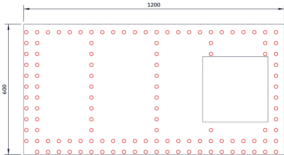
TOP VIEW
