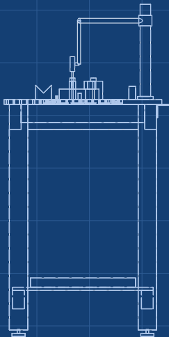
RIGHT VIEW Scale 1:20
