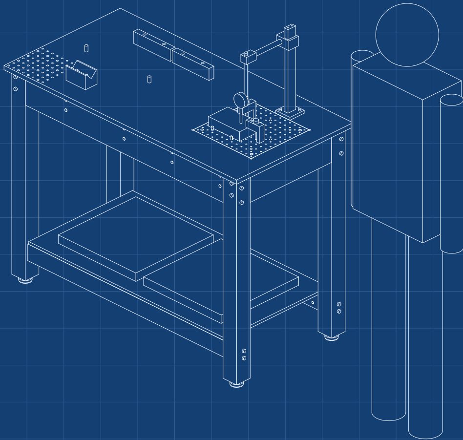
ISOMETRIC VIEW
