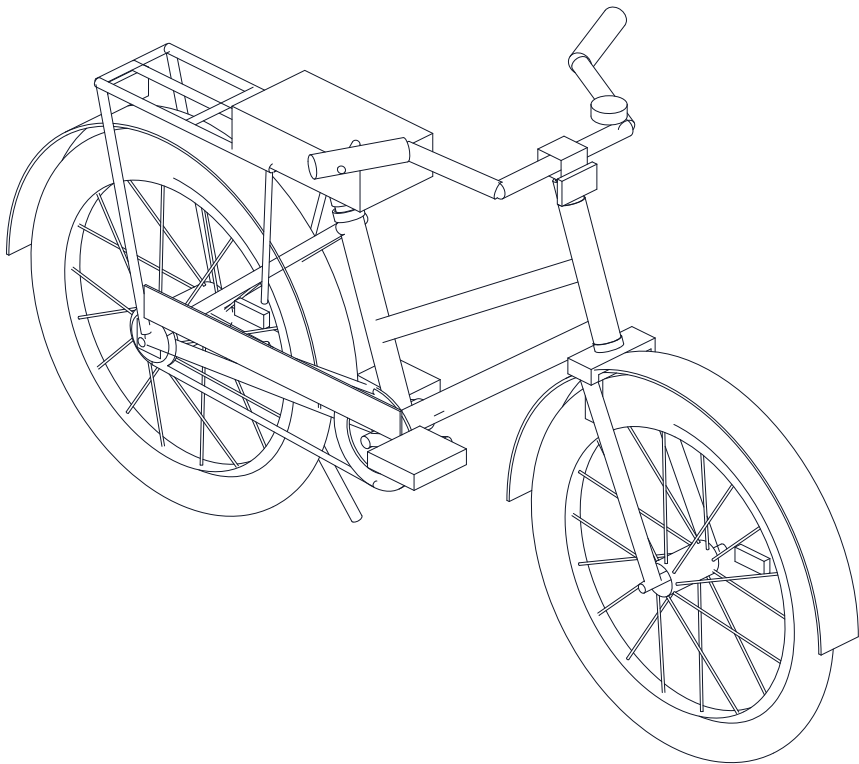
ISOMETRIC VIEW, SMALLEST RIDER SETTING Not to scale; seen from the front right and above, about 30 deg elevation
