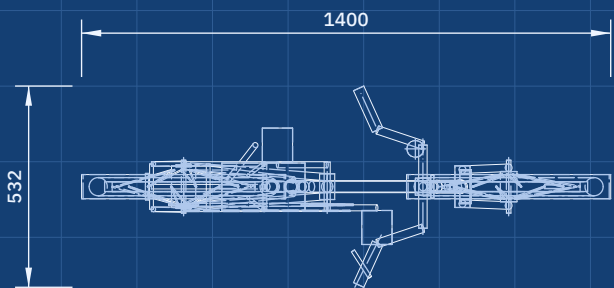
TOP VIEW Scale 1:20; looking down (along -Z)
