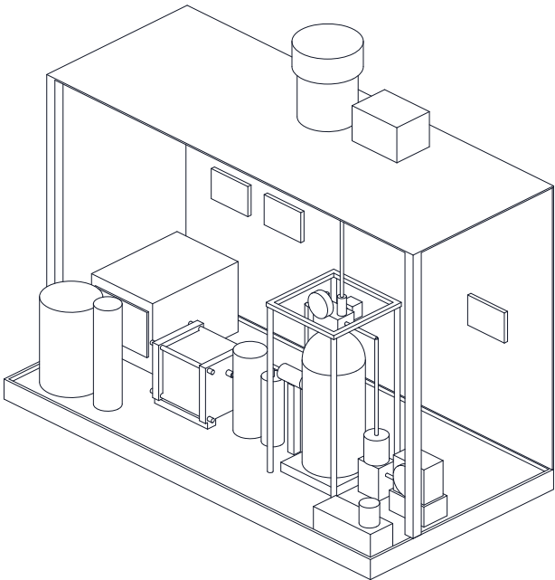
ISOMETRIC VIEW Not to scale; seen from the front right and above, about 30 deg elevation
