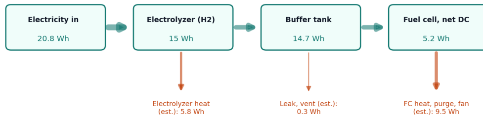
Figure 2. Energy per lesson cycle, HHV basis, from HBN-CAL-001. All values are paper estimates: electrolyzer 72.2 % (voltage efficiency 75.9 %, Faraday efficiency 95 %), 2 % lost to leaks and venting in storage, fuel cell 35.5 % net (0.60 V per cell, 95 % fuel utilization, 0.9 W fan and controls).
