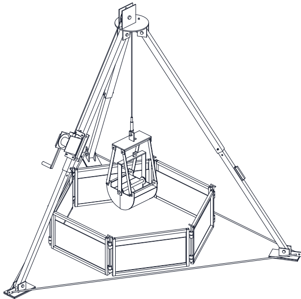
ISOMETRIC VIEW
