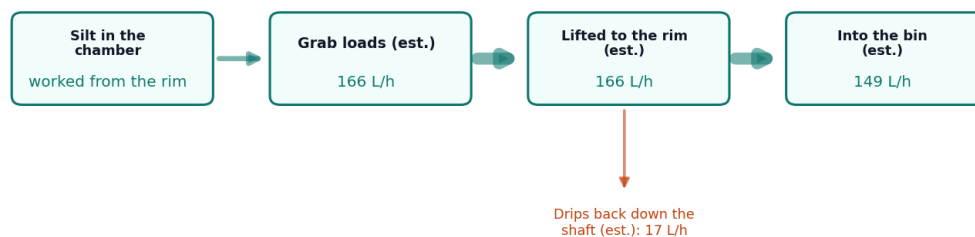
Figure 4. Silt removed per hour with the grab at 3 m depth (all values are estimates).
