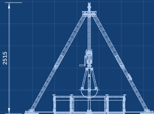
FRONT VIEW Scale 1:50; looking at the front (along +Y)
