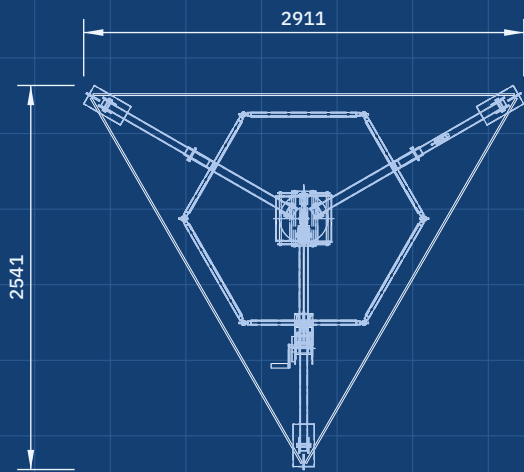
TOP VIEW Scale 1:50; looking down (along -Z)
