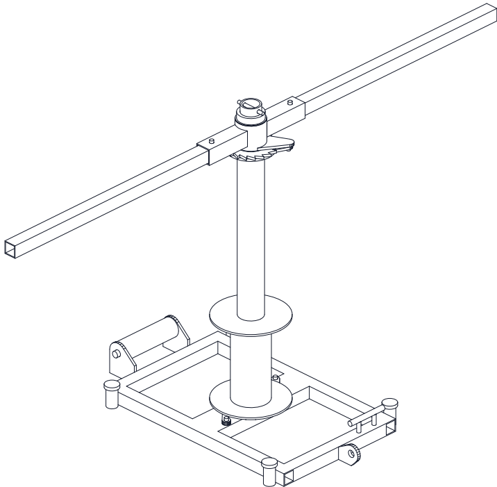
ISOMETRIC VIEW
