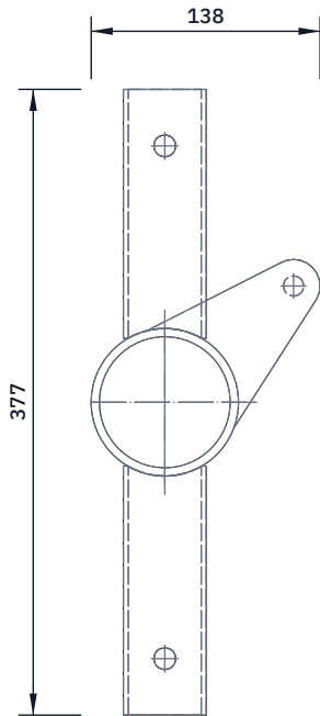
TOP VIEW
