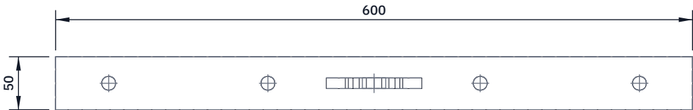
TOP VIEW Scale 1:5; looking down (along -Z)
