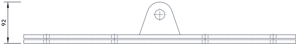
FRONT VIEW Scale 1:5; looking at the front (along +Y)
