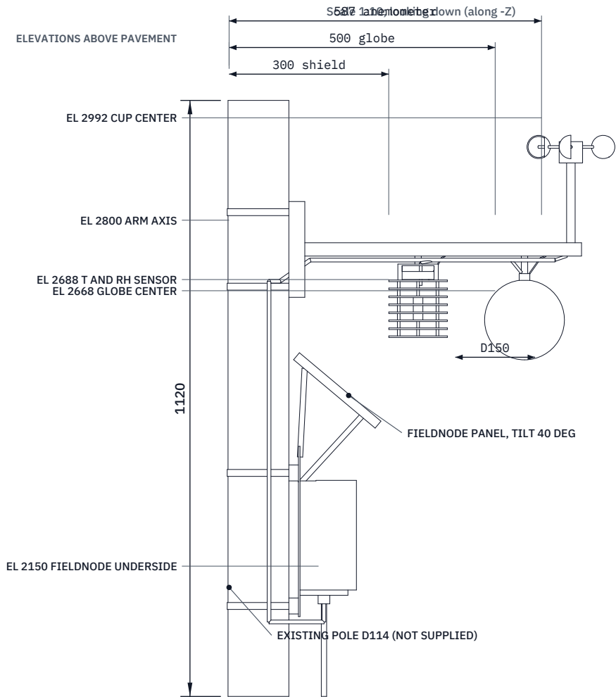
FRONT VIEW
