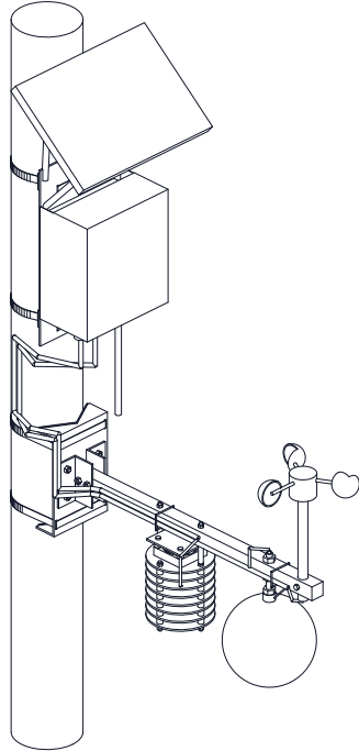
ISOMETRIC VIEW
