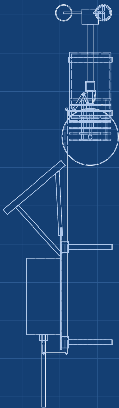
RIGHT VIEW Scale 1:10
