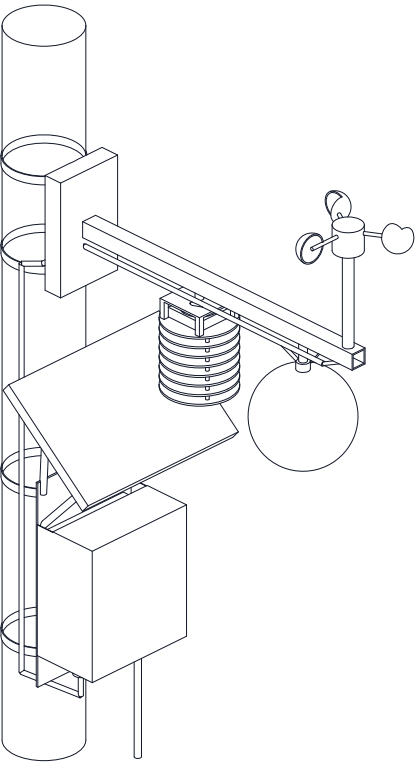
ISOMETRIC VIEW Not to scale
