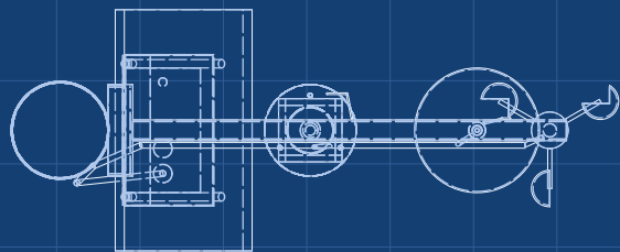
TOP VIEW Scale 1:10
