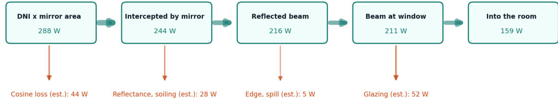
Figure 2. Instantaneous power from the sun to the room at the design point (DNI 800 W/m 2 , 10 m to the target, 32° incidence), in W. Values from HLT-CAL-001 [A2]; all are estimates.
