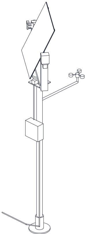
ISOMETRIC VIEW, TRACKING POSE Not to scale; seen from the front right and above, about 30 deg elevation
