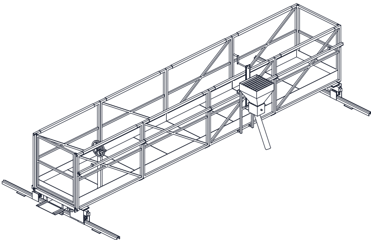
ISOMETRIC VIEW
