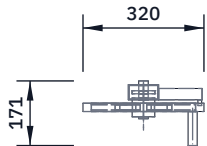
TOP VIEW Scale 1:20; looking down (along -Z)
