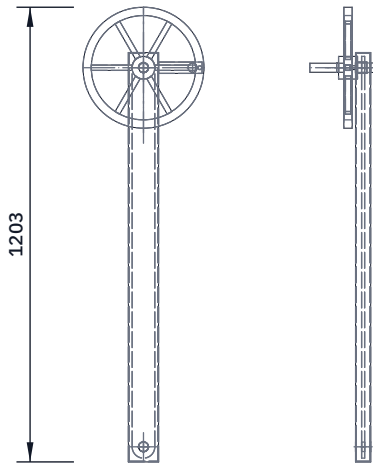
FRONT VIEW Scale 1:20; looking at the front (along +Y) RIGHT VIEW Scale 1:20; looking at the right side (along -X)
