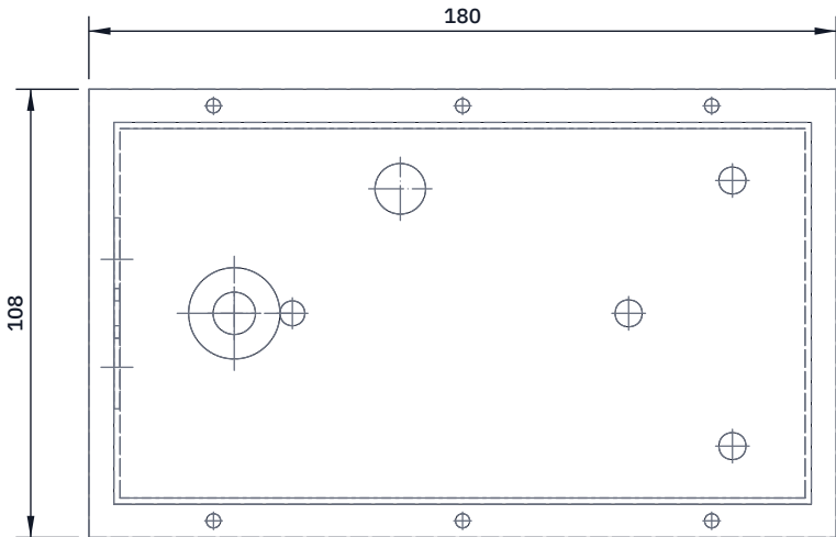
TOP VIEW Scale 1:2; looking down (along -Z)
