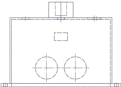
RIGHT VIEW Scale 1:2; looking at the right side (along -X)
