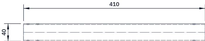
TOP VIEW Scale 1:5; looking down (along -Z)
