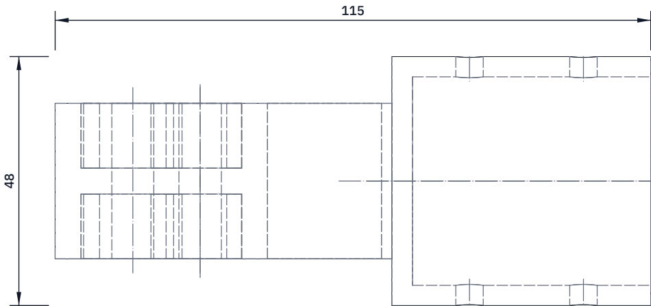
TOP VIEW Scale 1:1; looking down (along -Z)
