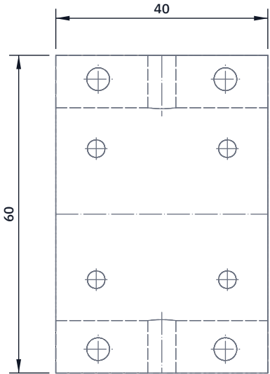
TOP VIEW Scale 1:1; looking down (along -Z)
