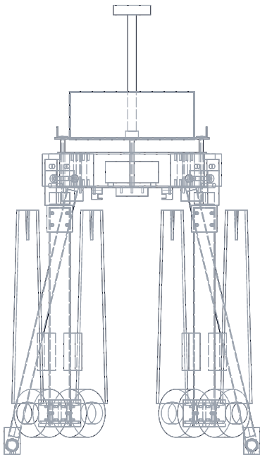
RIGHT VIEW
