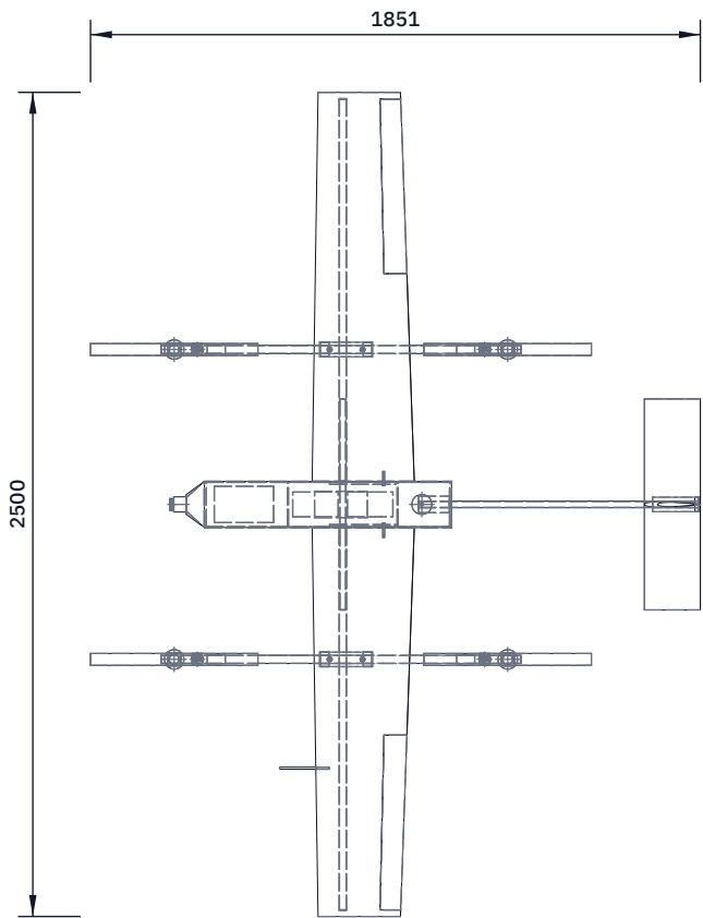
TOP VIEW
