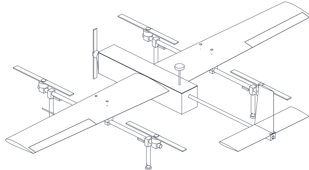
ISOMETRIC VIEW
